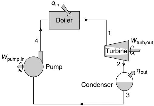
Fig. 4.5 Rankine Cycle
