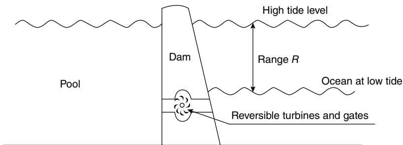
Fig. 1.6 A Tidal Energy Harnessing Plant
