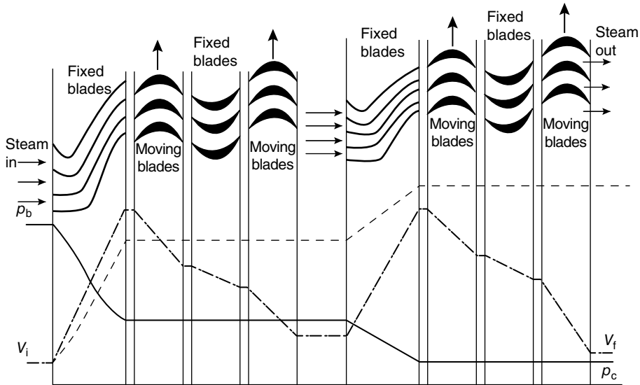
Fig. 10.7 Pressure–Velocity Compounding
