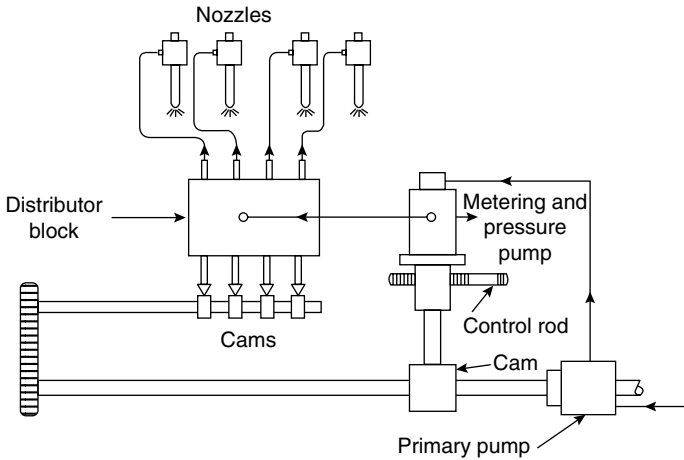
Fig. 13.12 Distributor System
