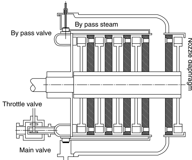
Fig. 10.20 Bypass Governing
