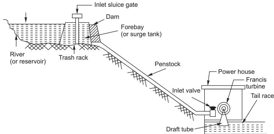
Fig. 2.1. Layout of Hydroelectric Power Plant
