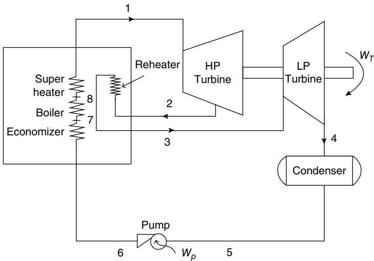
Fig. 4.17 Reheat Cycle
