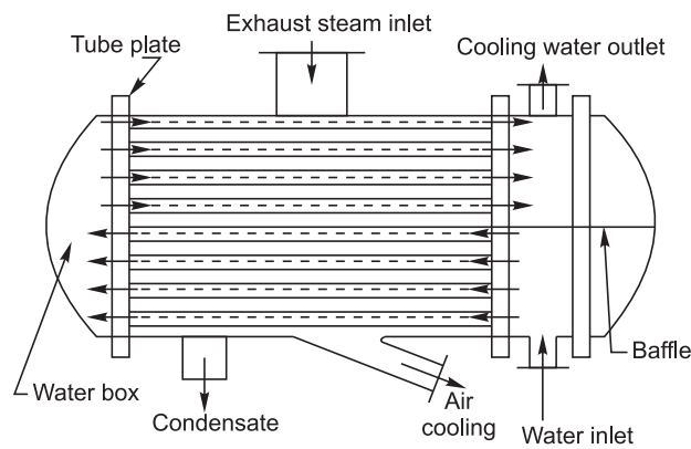
Fig. 1.23. Surface Condenser
