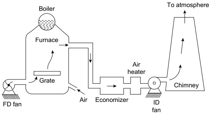
Fig. 7.3 Balanced Draught
