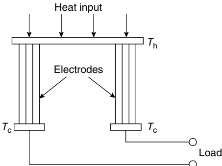
Fig. 1.12 Thermoelectric Generator
