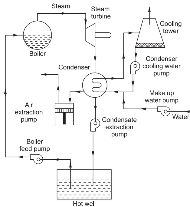
Fig 1.18. Steam Condensing plant
