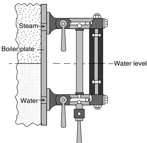
Fig. 5.32 Water-Level Indicator
