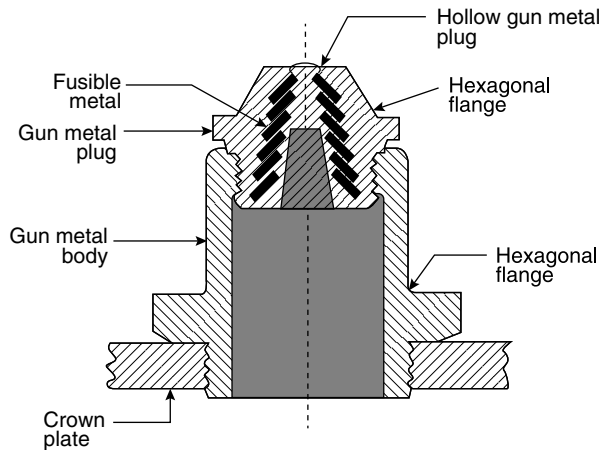
Fig. 5.37 Fusible Plug
